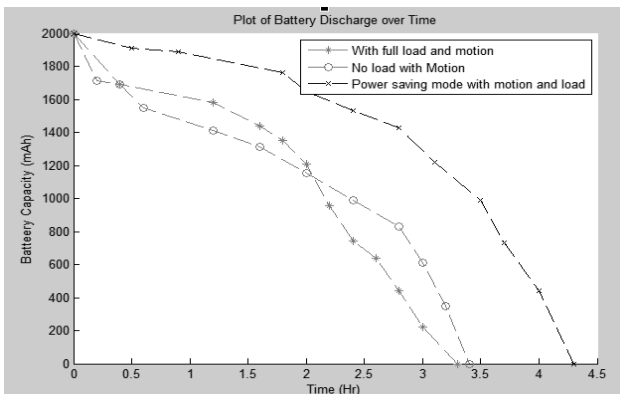
Fig. 11 – Battery Capacity Vs Operating Time for Rover 5.
