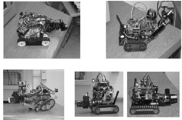
Fig. 13 – UB Swarm of Robots.
