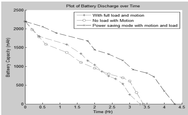
Fig. 8 – Battery Capacity Vs Operating Time for Rover 2.
