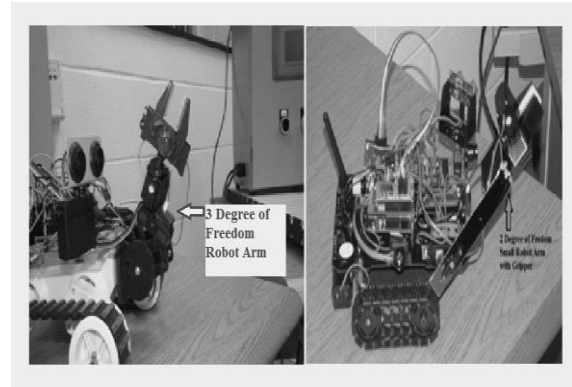
Fig. 6 – Manipuator with Gripper.
