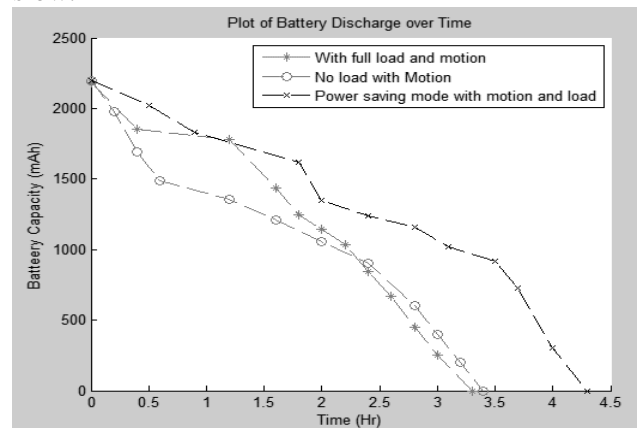
Fig. 7 – Battery Capacity Vs Operating Time for Rover 1.
