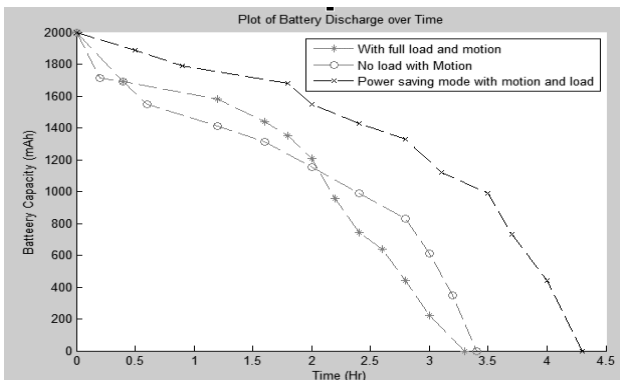
Fig. 10 – Battery Capacity Vs Operating Time for Rover 4.
