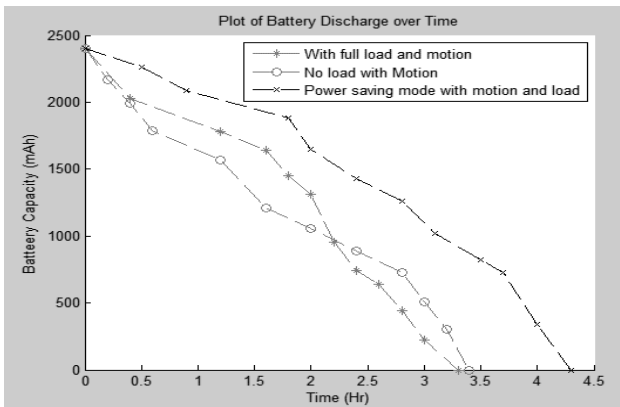
Fig. 9 – Battery Capacity Vs Operating Time for Rover 3.
