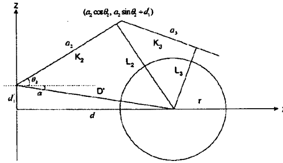
FIGURE 3 Link intersection with the XZ Plane.
