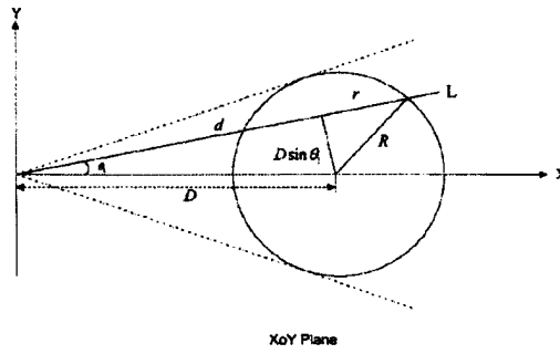
FIGURE 2 Link intersection with the XY Plane.
