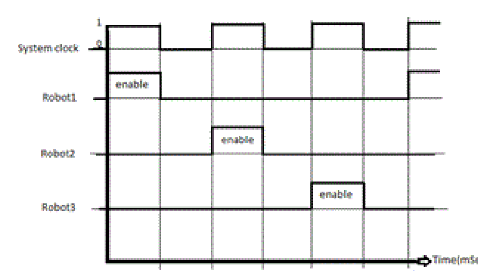
Figure 5: System clock need to allow data transmission to avoid interfering.
