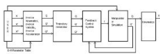
Figure 11. Block diagram for the simulation package
